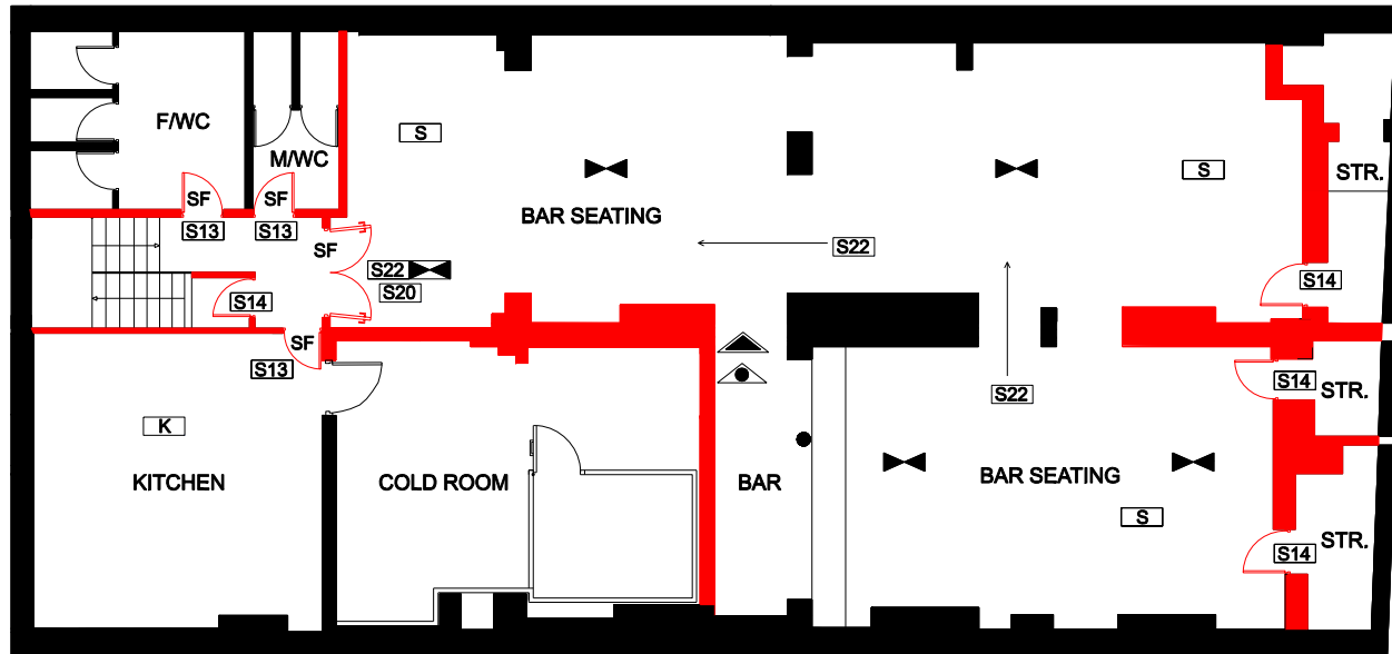
02 / BASEMENT PLAN
